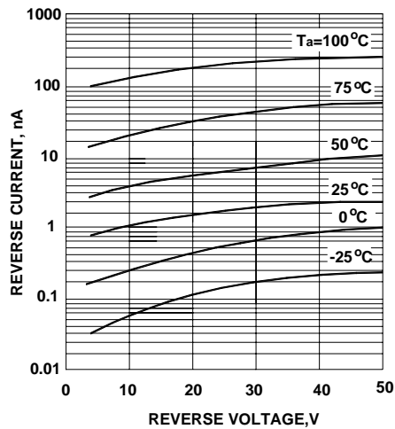
REVERSE CHARACTERISTICS
